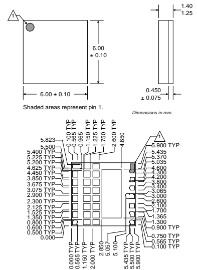
Package Style: Module, 6mm x 6mm
