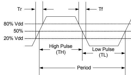
Figure 3. Output Waveform
