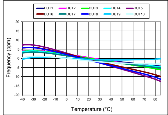
Figure 9. Frequency vs Temperature, 1.8V
