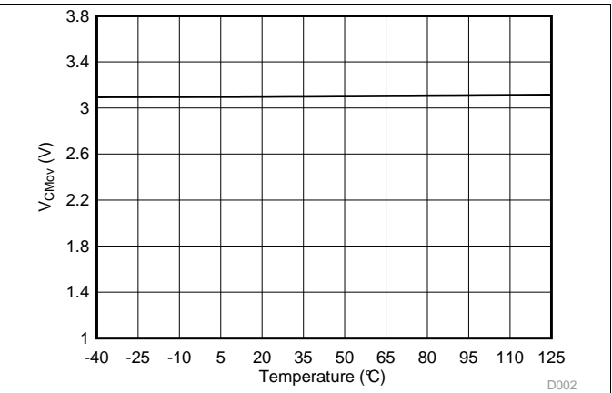
Figure 5. Common-Mode Overtolerance Detection Level vs Temperature
