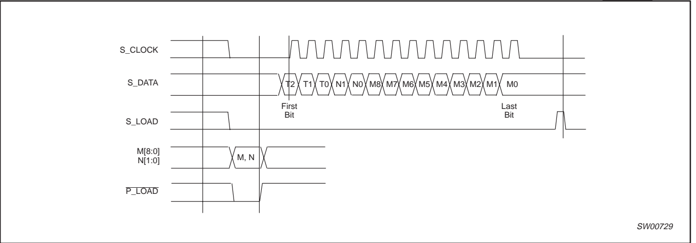
Figure 1. Timing Diagram
