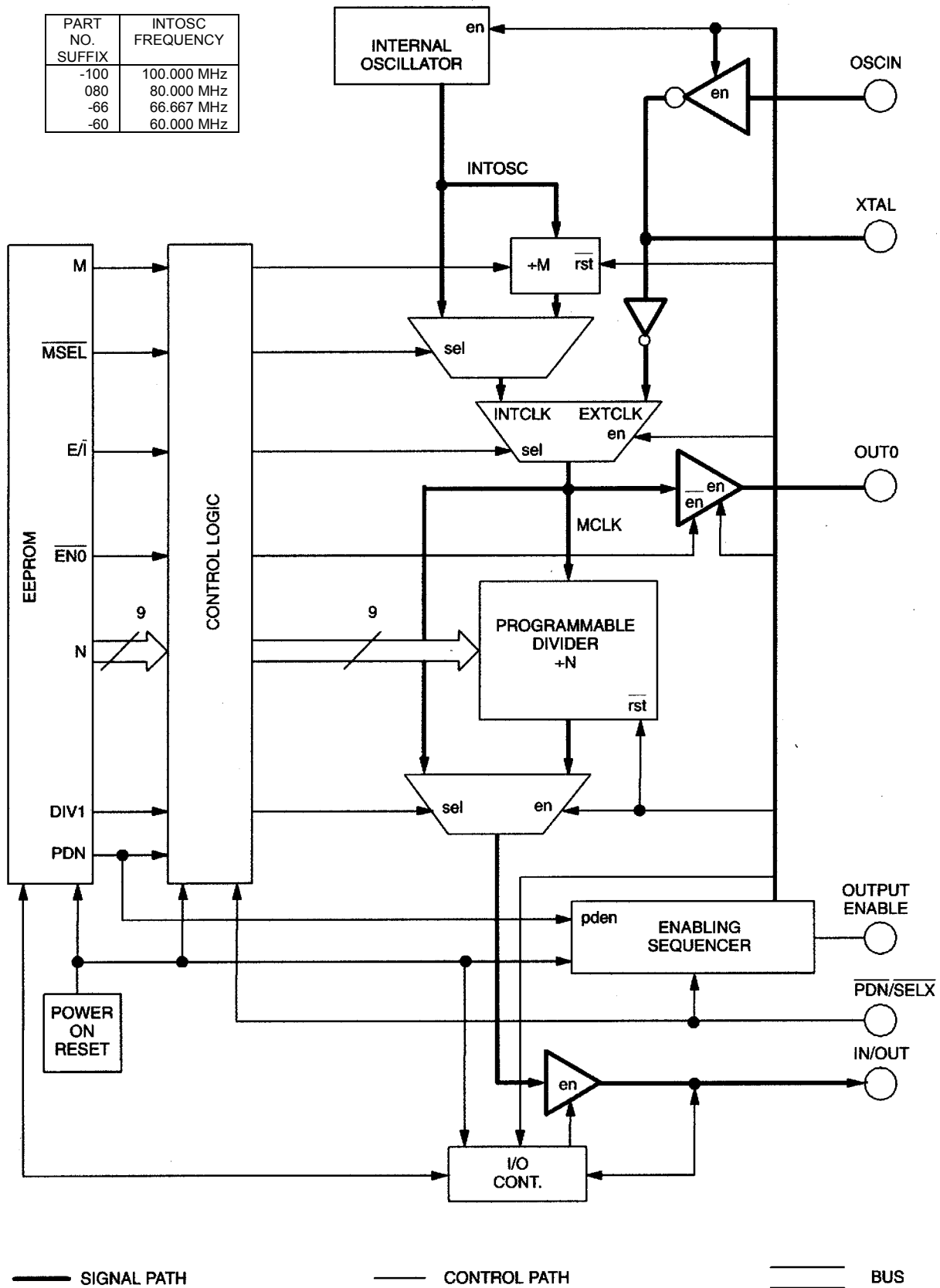
BLOCK DIAGRAM Figure 1
