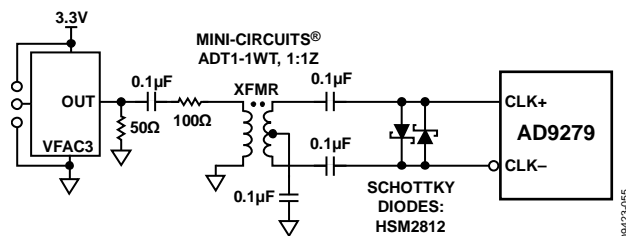
Figure 53. Transformer-Coupled Differential Clock
