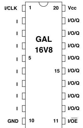
DIP
