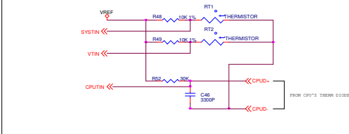
Temperature Sensing
