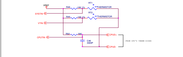
Temperature Sensing
