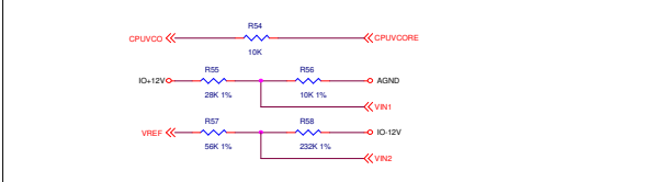
Voltage Sensing
