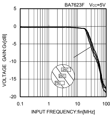
Fig.10 Frequency characteristic vs. Temperature
