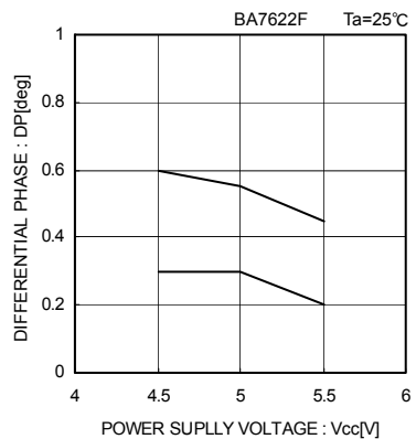
Fig.40 Differential phase (clamp) vs. Supply voltage
