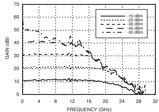
Response vs. Input Power [1][4][5]
