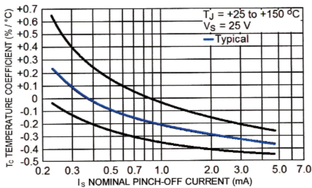
FIGURE 2 – TEMPERATURE COEFFICIENT
