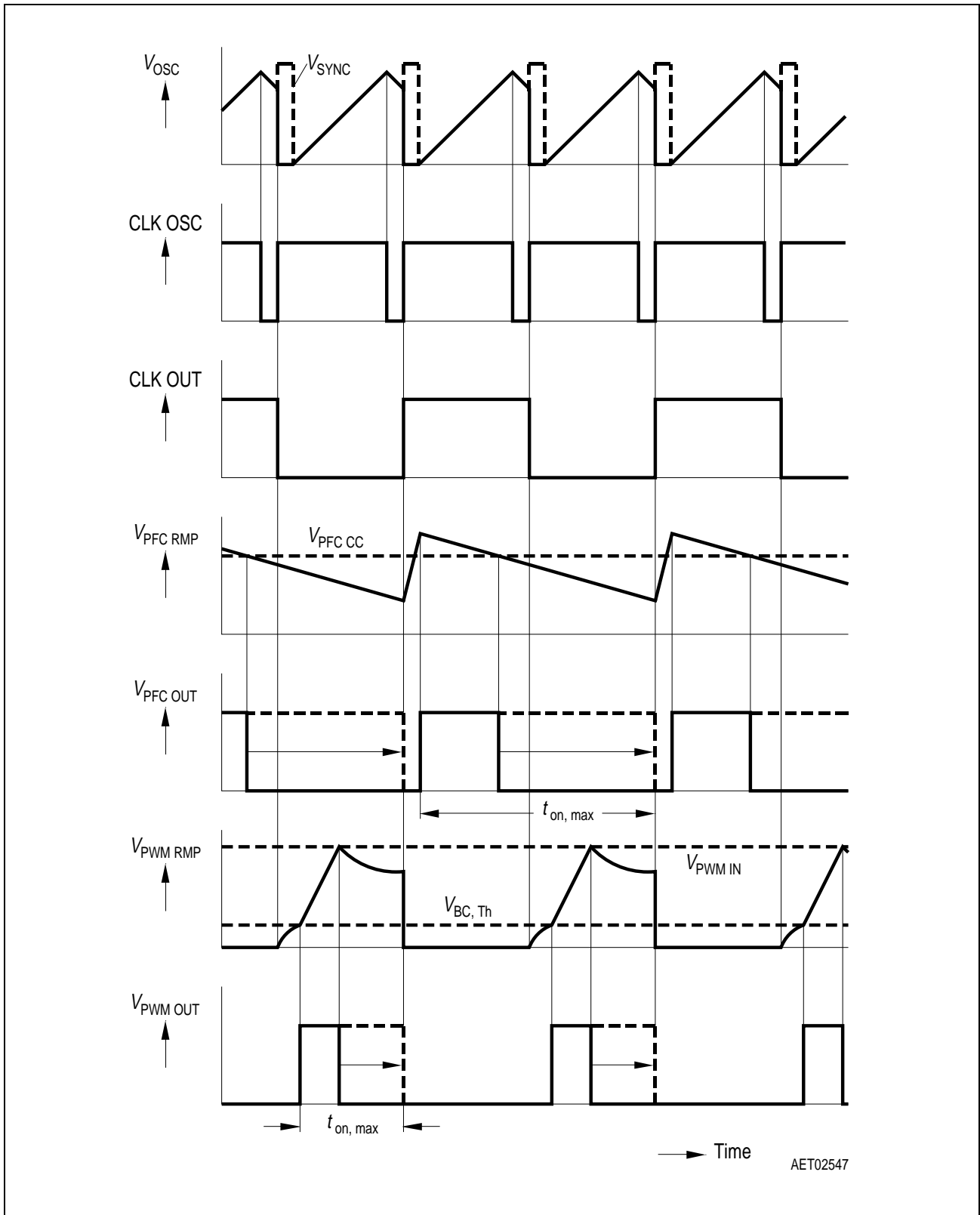
Figure 19 Timing Diagram with Synchronization ( f_{\text{SYNC}} > f_{\text{osc}} )
