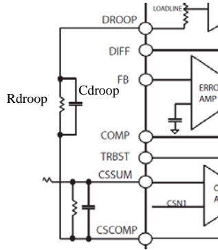
Figure 12. Droop RC
