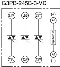
Terminal Arrangement/Internal Circuit Diagram
