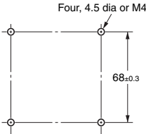
Mounting Holes
