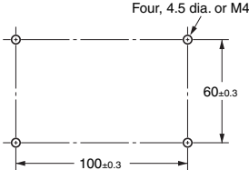
Mounting Holes
