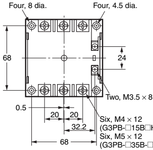
Without Terminal Cover
