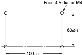
Mounting Holes
