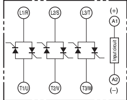
G3PB-445B-3-VD
