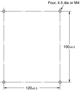
Mounting Holes
