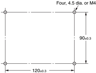
Mounting Holes
