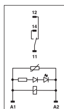
AC coils
