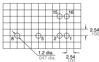
Terminal No.2 and 15 are for DSP1a-PSL2 only.
