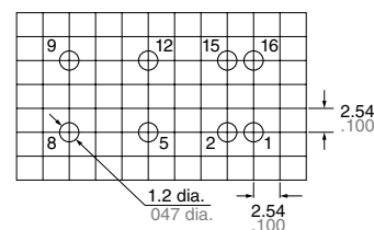
Terminal No.2 and 15 are for DSP2a-PSL2 only.
