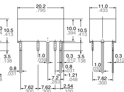
2 coil latching
