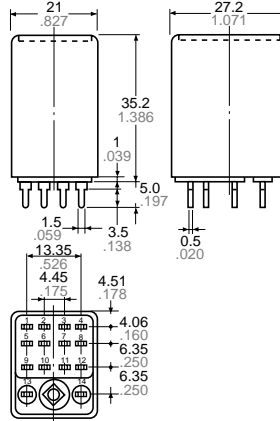
External dimensions
