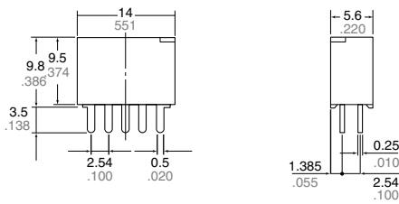
Self-clinching terminal
