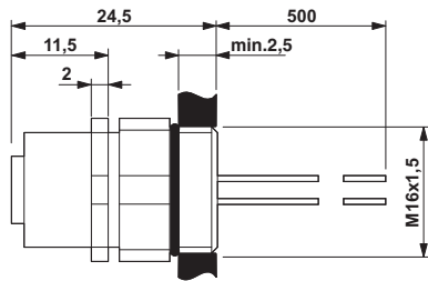
M12 flush-type connector, can be positioned
