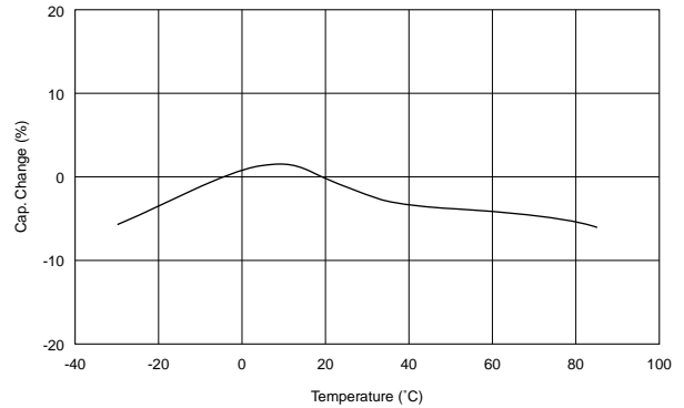
B Characteristics
