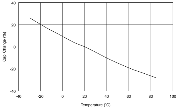
ZM Characteristics
