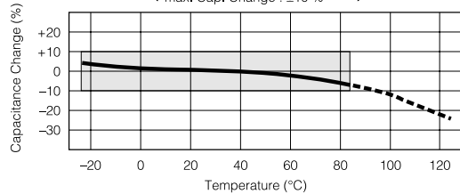
Series HT-KB, KBP (Char. B/Y5P)
