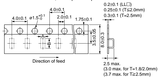
8mm width, 4mm pitch Tape
