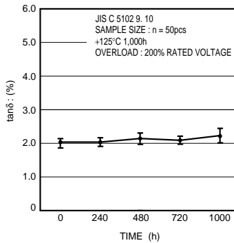
Fig.20 tanδ
