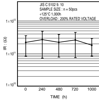
Fig.21 Insulation resistance
