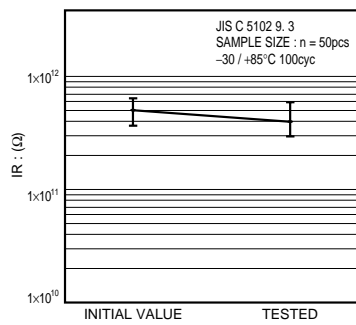
Fig.15 Insulation resistance
