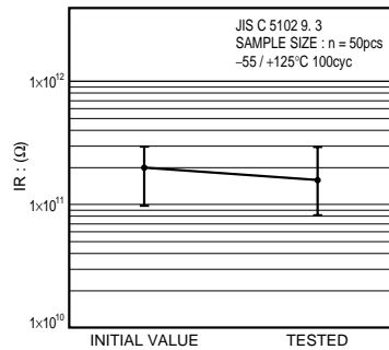
Fig.12 Insulation resistance
