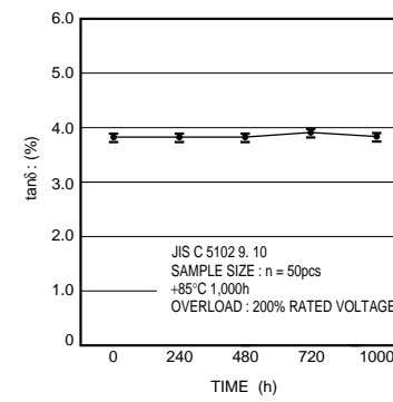
Fig.23 tanδ
