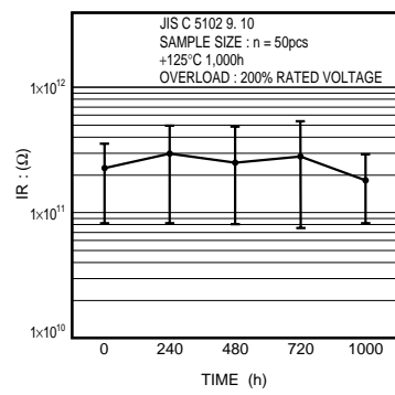
Fig.21 Insulation resistance
