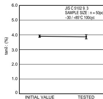
Fig.14 tanδ
