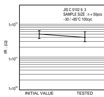
Fig.15 Insulation resistance
