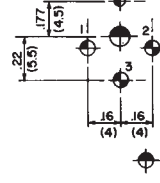
Component Side Layout
