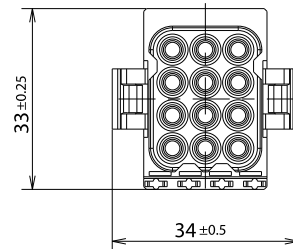
Plug, 12 poles
