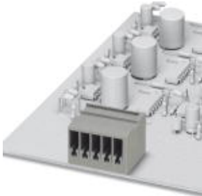
ST-COMBI receptacle, plug-in direction horizontal to the PCB, pitch: 5.2 mm, no. of positions: 10
