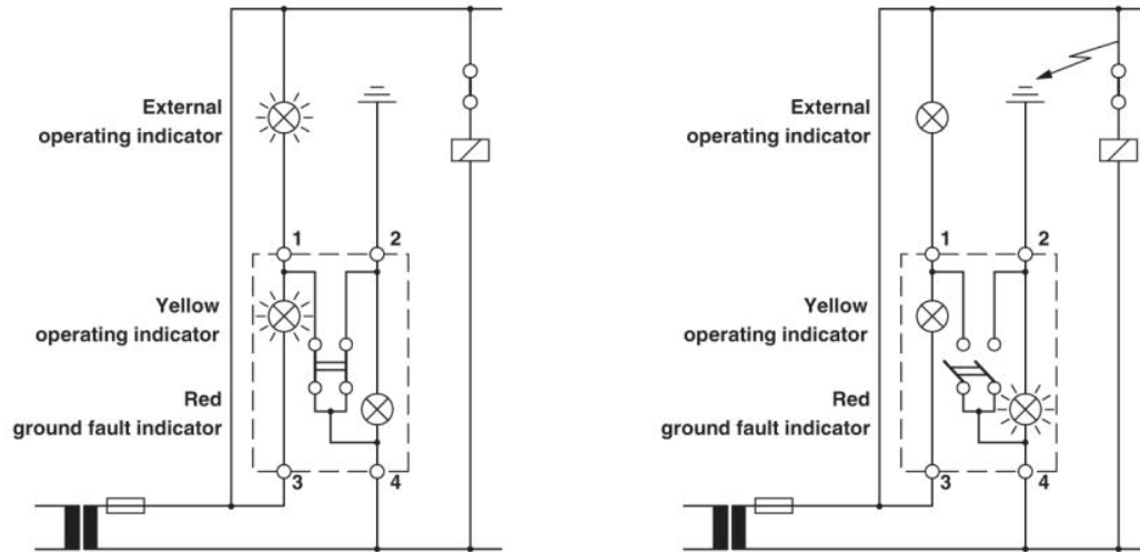
Circuit diagram
