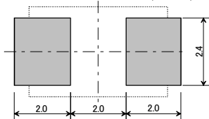
REFERENCE LAND PATTERN (TYPICAL)
