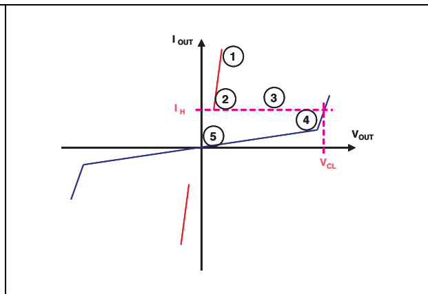
Figure 18. Description of the different steps during switching off of a high inductive load
