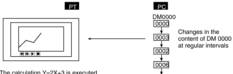
The calculation Y=2X+3 is executed continuously in the PT and the results are displayed in the trend graph.
