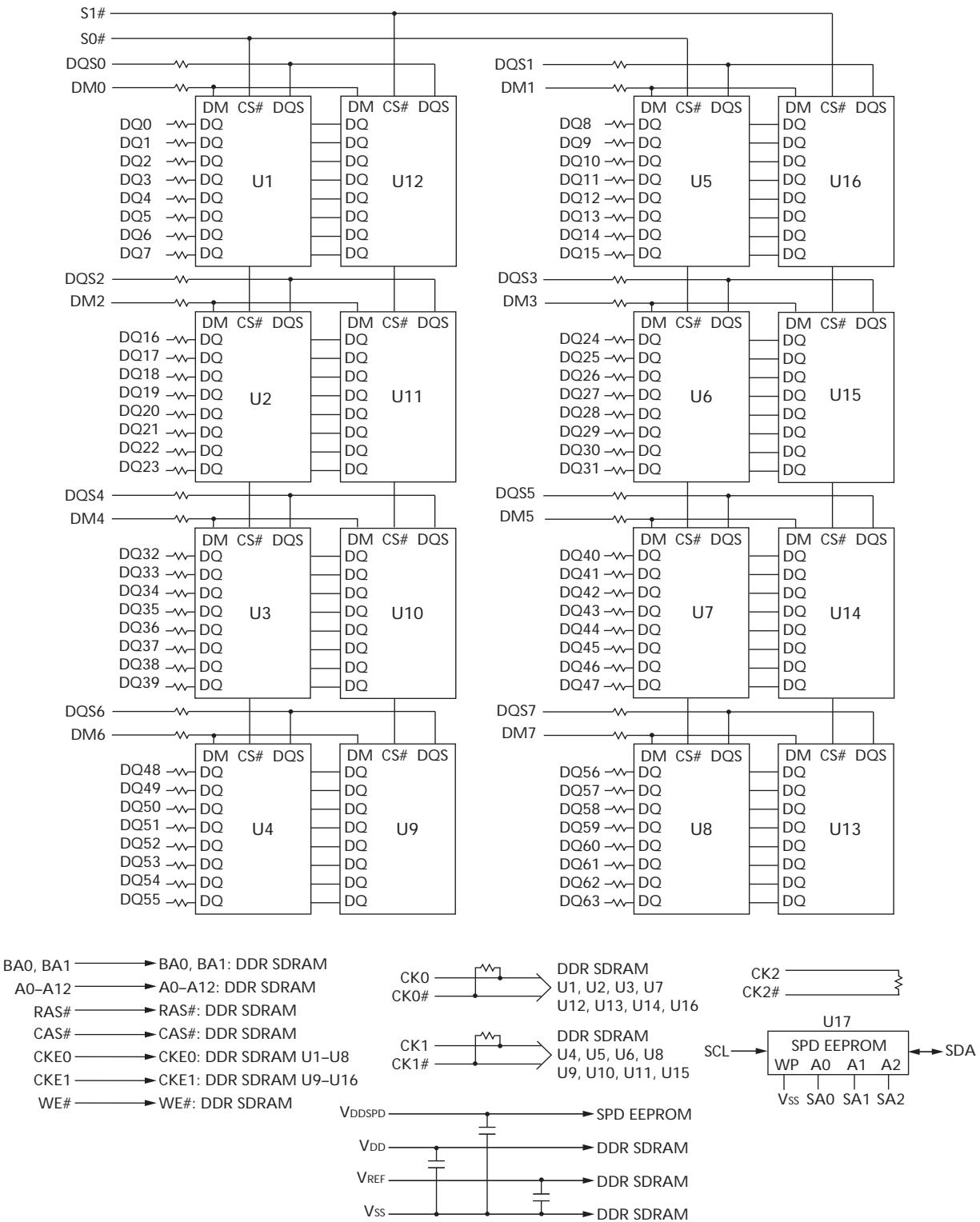
Figure 4: Functional Block Diagram - 1GB
