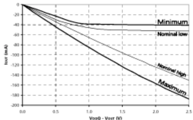
Figure 8: Pull-Up Characteristics
