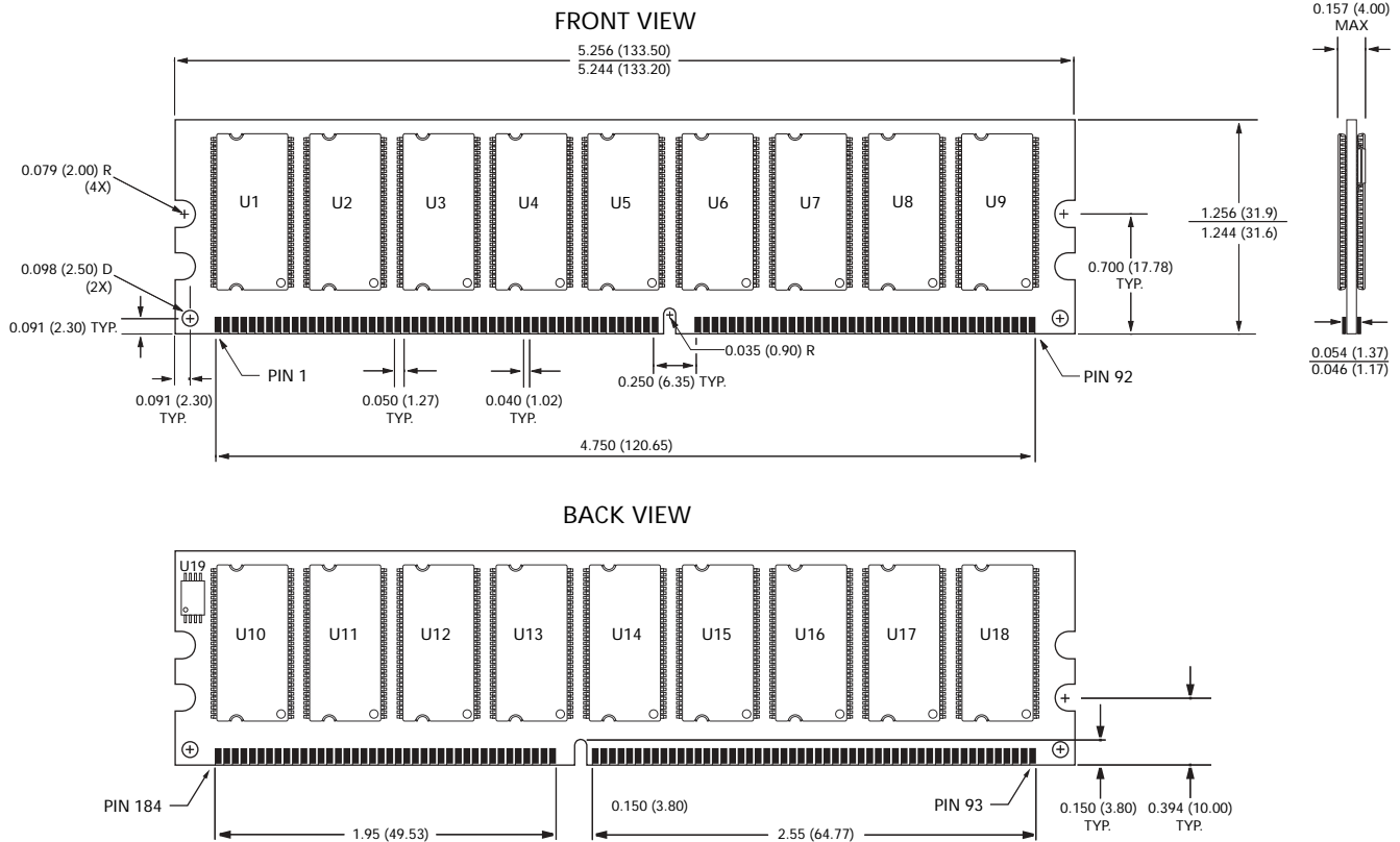
Figure 15: 184-PIN DIMM Dimensions
