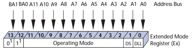
Figure 6: Extended Mode Register Definition Diagram
