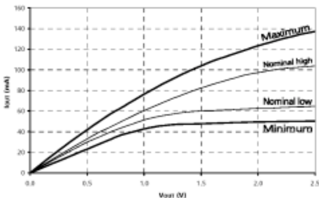
Figure 7: Pull-Down Characteristics
