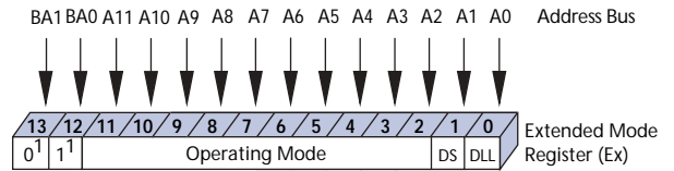
Figure 6: Extended Mode Register Definition Diagram
