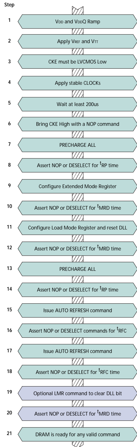
Figure 9: Initialization Flow Diagram
