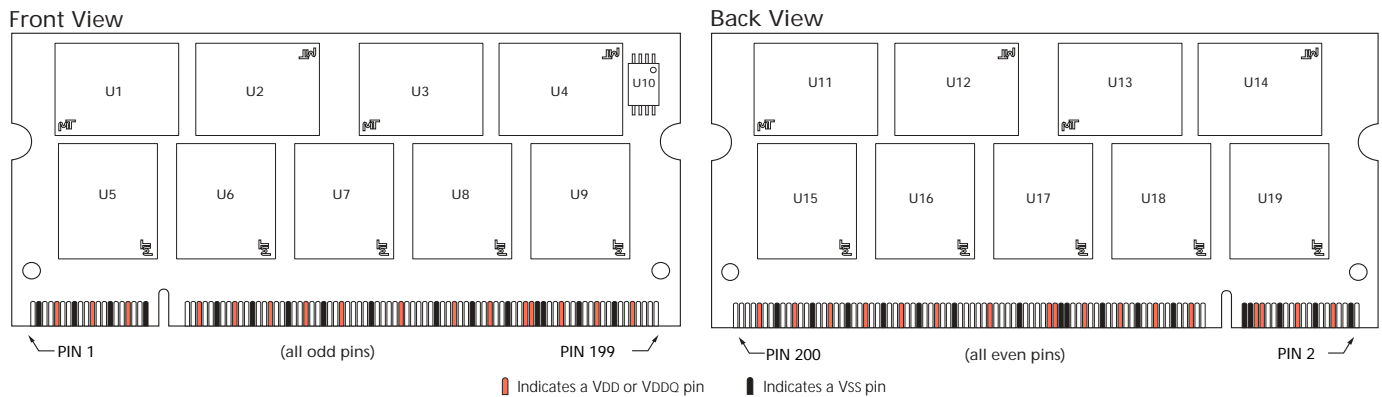
Figure 2: Module Layout
