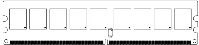
Figure 1: 240-Pin UDIMM (MO-237 R/C G or RC/ B)
