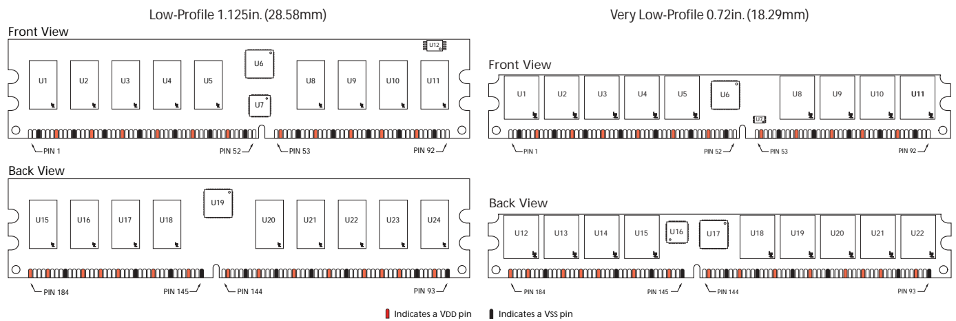
Figure 2: Pin Locations
