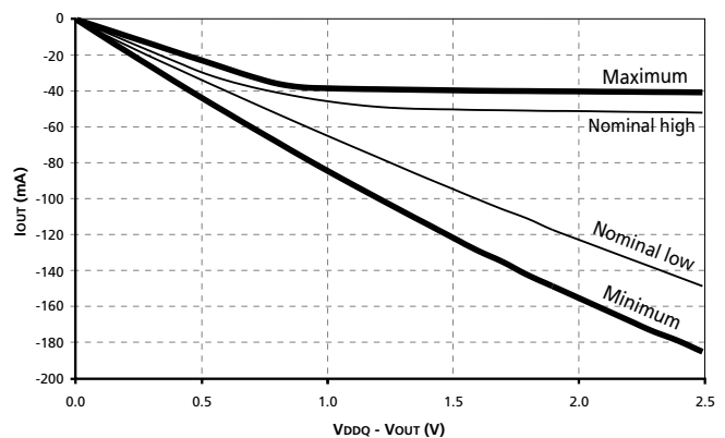
Figure 10: Pull-Up Characteristics
