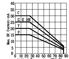
Fig8. MAX ALLOWABLE DC CURRENT VS. AMBIENT TEMPERATURE.
