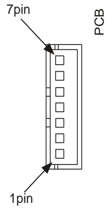
RS-232 interface connector JST: B7B-XH-A or equivalent
