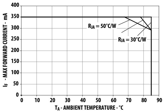
Figure 5. Maximum forward current vs. ambient temperature for AllnGaP Derated based on T_{jMAX} = 110^{\circ}C , R_{\theta JA} = 30^{\circ}C/W / 40^{\circ}C/W and 50^{\circ}C/W
