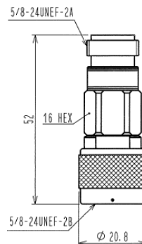
N Type AT-400
