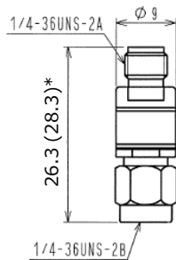
SMA Type (Plug - Jack) AT-100V
