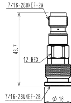
TNC Type AT-600
