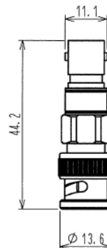
BNC Type AT-500
