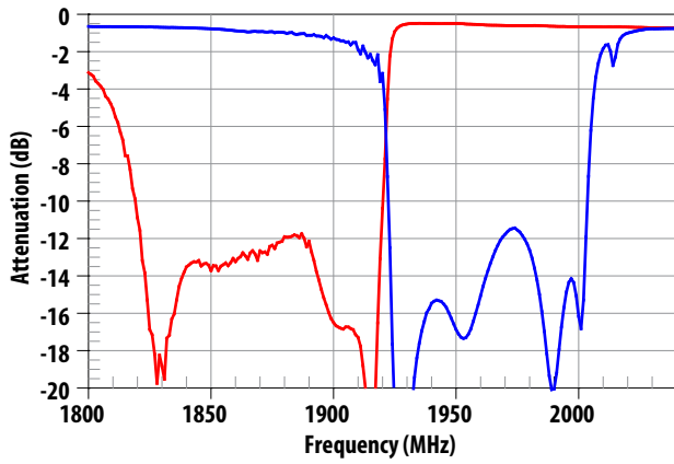
Figure 5. PCS Tx and Rx Port Return Loss (Dual Antenna, Note1).
