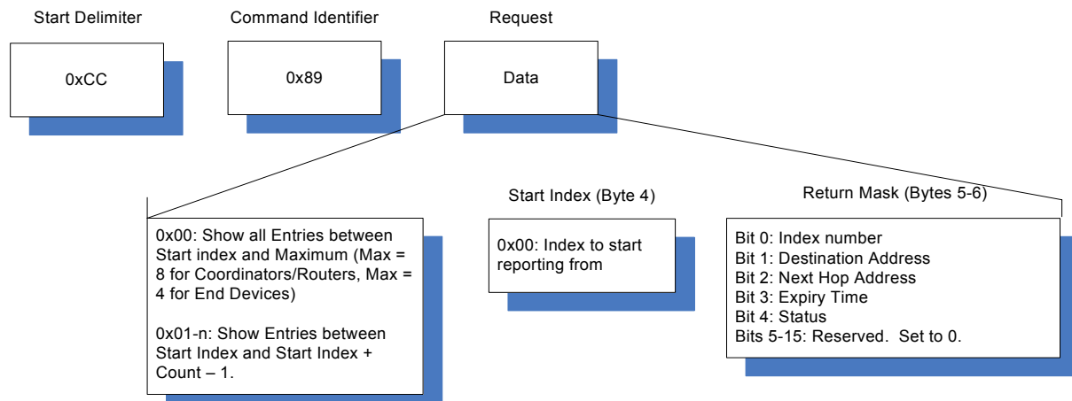
Figure 19: Read Route Table Command
